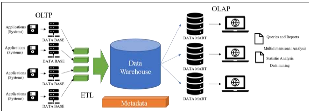
Figure 2. Traditional BI with Data Warehouse.
